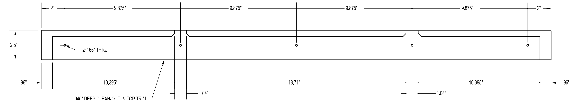
TOP TRIM BACK VIEW SCALE 1/4" = 1"
