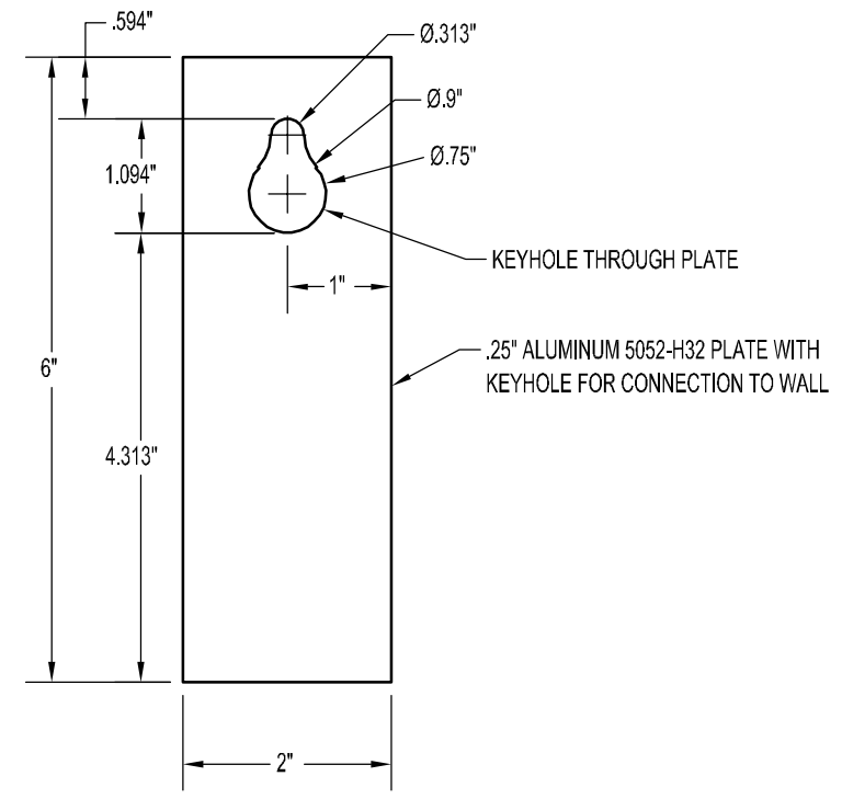
KEYHOLE PLATE SCALE 1/2" = 1"
