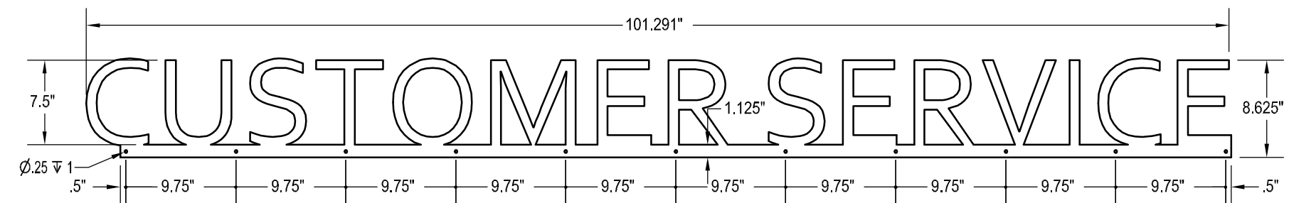
FRONT VIEW SCALE 1" = 1'
