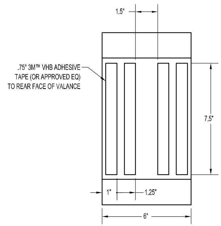
FRONT VIEW SCALE 1/4" = 1"
