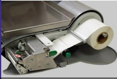
Pull out Printer - for easy label loading.
