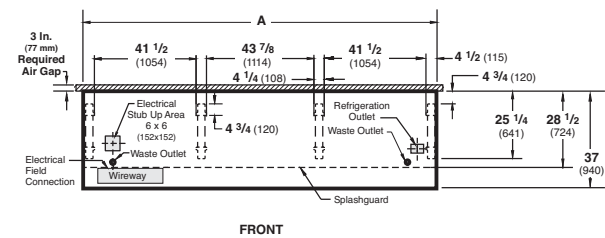
Plan View - D5NX-LE, D5NX-LEP
